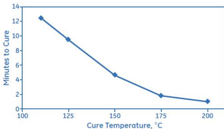
Figure 1: Addisil 6101 Silicone Adhesive Cure Time vs Temperature
